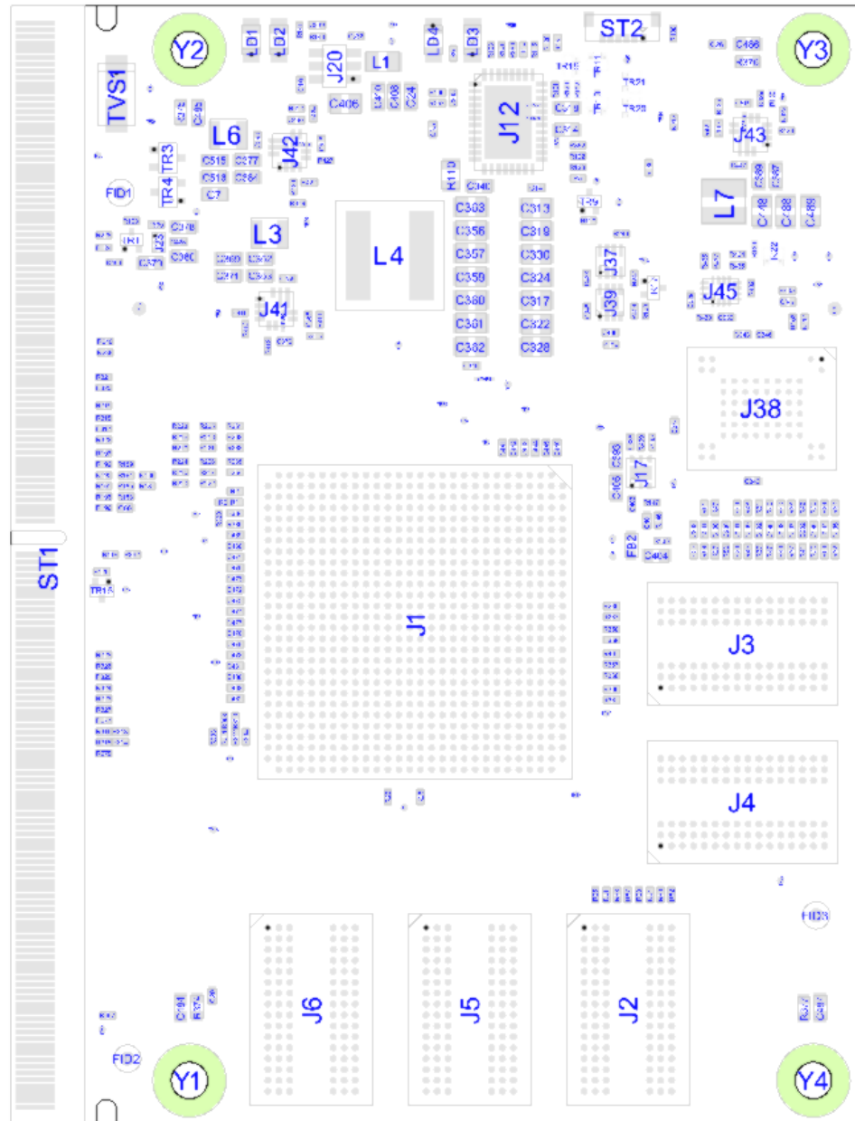
Figure 5-7 Top Components
