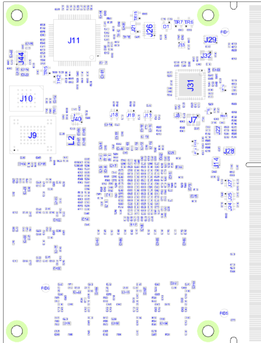
Figure 5-8 Bottom Components
