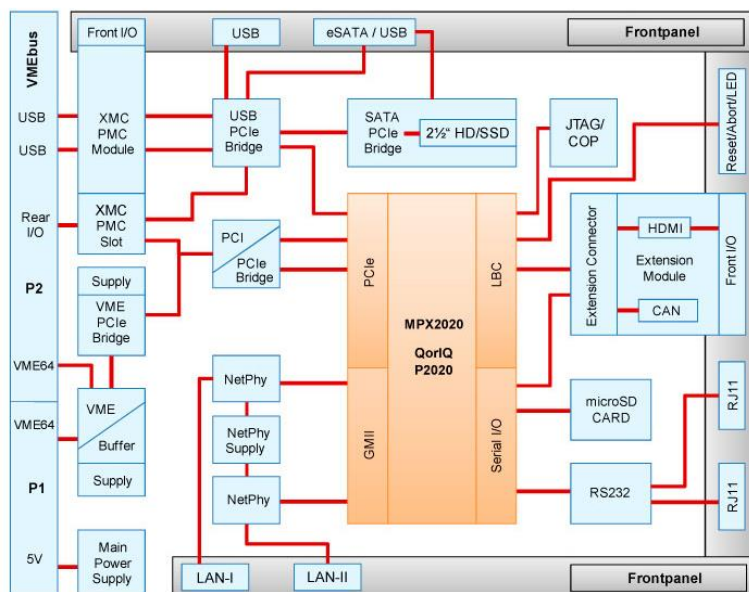
Fig. 1 Block diagram
