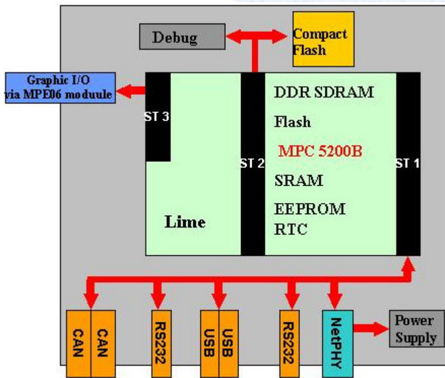
Block Diagram CRX02
